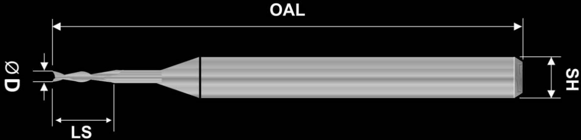
S.C. 2 / 4 Flute TiAlN / AlCrN COATED End Mill
